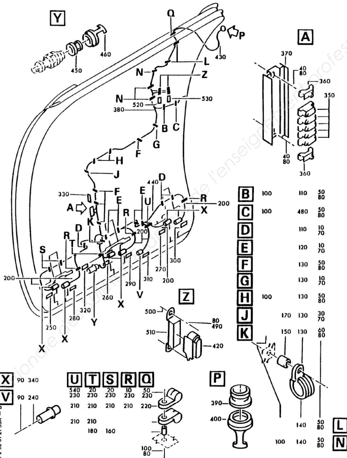
FIGURE 53A / 52-31-21 ROUTING INSTL- ** ON A/C ALL
