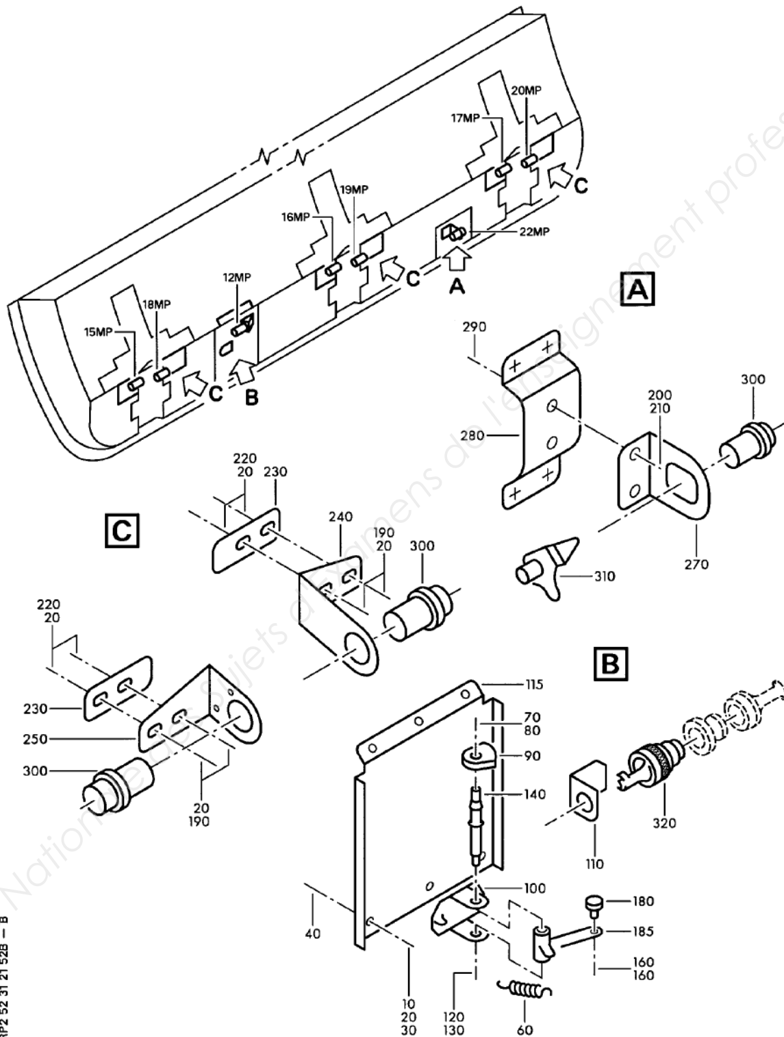
FIGURE 52B / 52-31-21 MICROSWITCHES INSTL- ** ON A/C ALL
