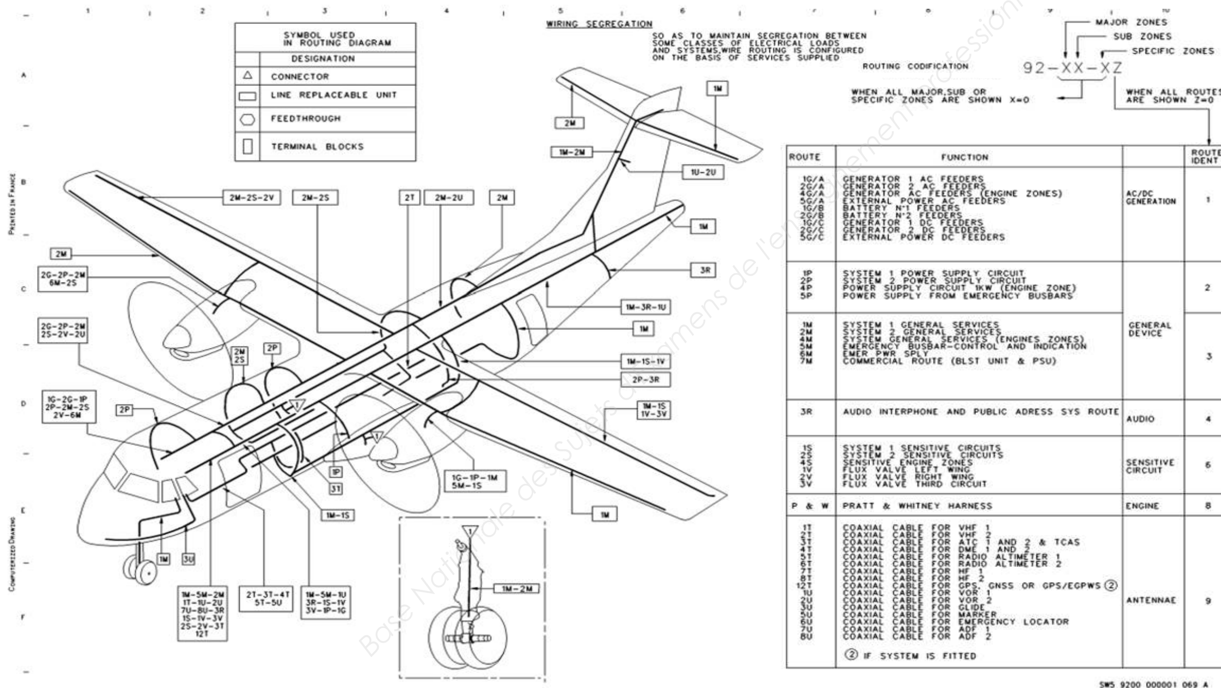
92-00-00 P 005 Figure 1 - ELECTRICAL ROUTING MAIN ROUTING & ROUTES IDENT ** ON A/C
